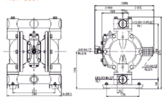
NDP-25BF
