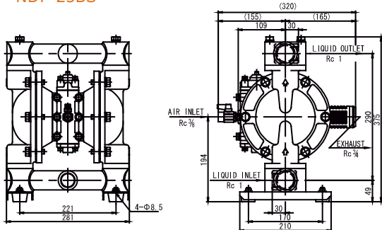
NDP-25BS
