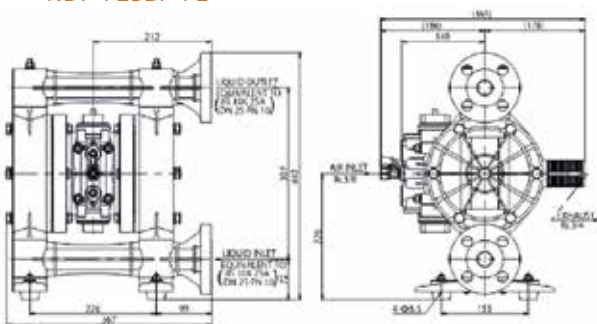
NDP-P25BP-FL
