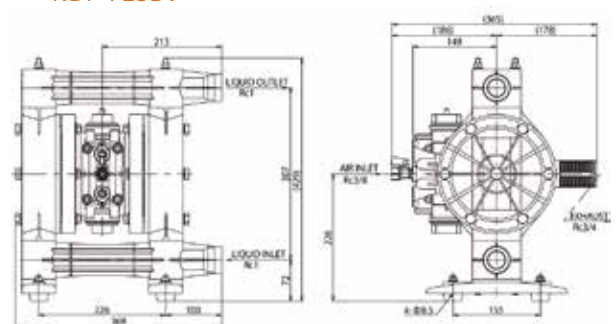
NDP-P25BV
