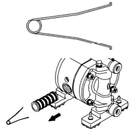
713148—Sleeve remover
